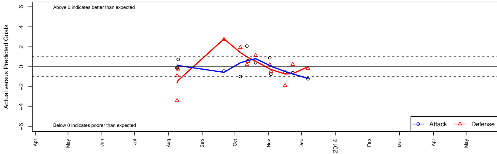
Sunnyvale Alliance SC Bulls Red B02 Dots are actual minus expected GF (blue circles) and GA (red triangles). Blue line is smoothed change in attack strength. Red is smoothed change in defense strength.
